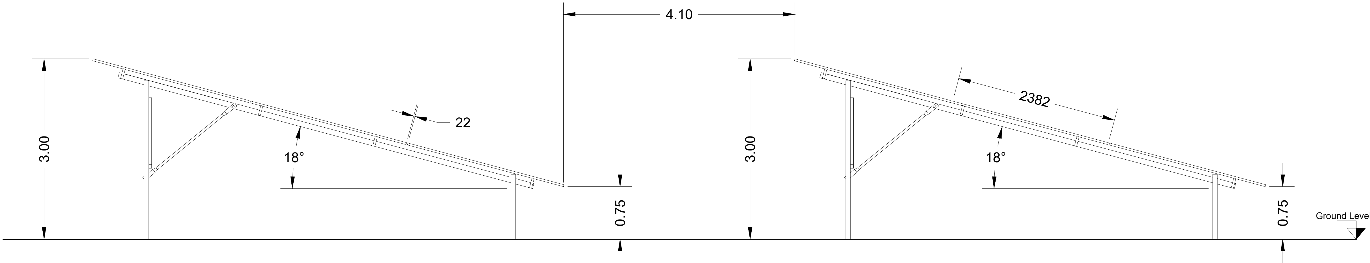
PV Mounting Structure Elevation (3 Portrait)
